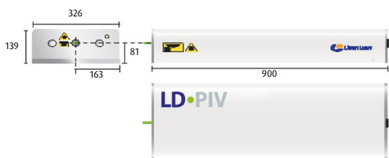
PIV Laser Head
